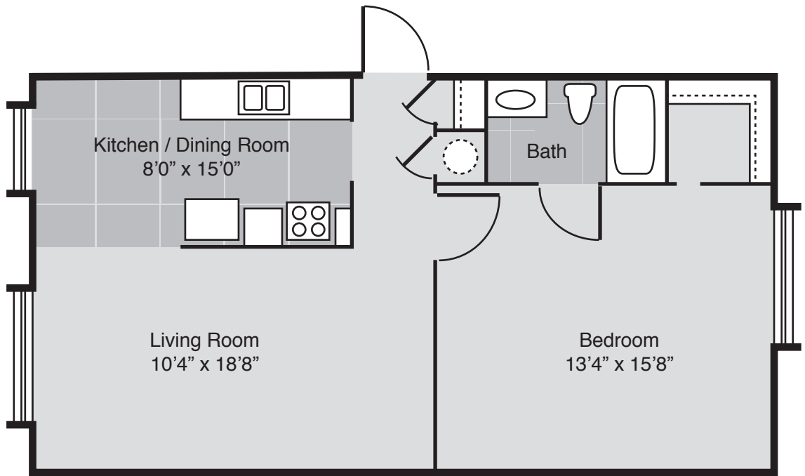
Unit A - One Bedroom - One Bath 720 Square Feet
